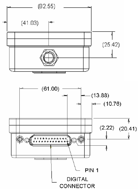
END VIEWS
