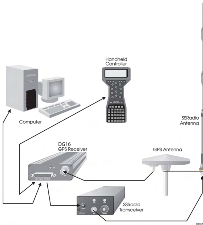
Figure 8.1. RTCM Base Station System
