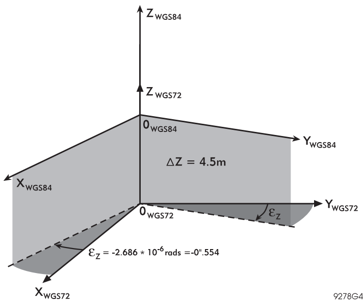
Figure 4.8. Rotation & Translation Between WGS-72 & WGS-84
