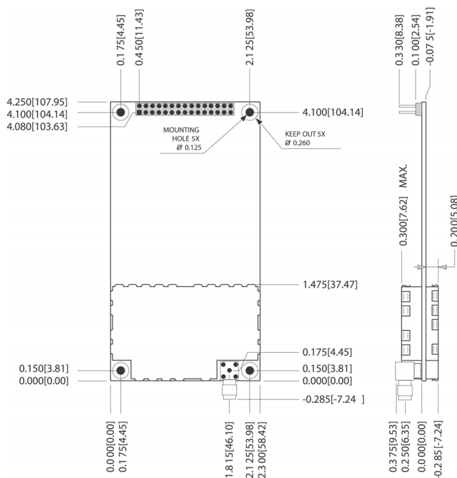
Figure 1.1. DG16 and DG14 GPS Board Dimensions—inches [mm]
