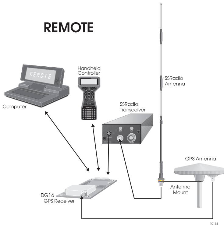
Figure 8.2. RTCM Remote System
