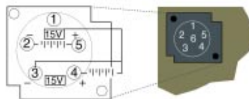
Connector Pin Schematic
