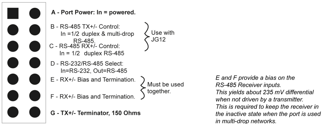
Figure 3: Port Control, Group B (ports 5 to 8)
