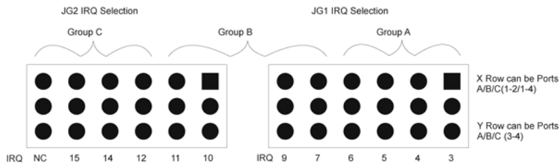
Figure 6: IRQ Selection, JG1 and JG2
