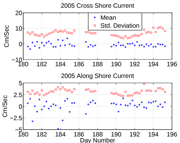
Fig. 14. 6 Hour Current Statistics at 1.8 Meter Altitude. 10 second wave motion is averaged out.
