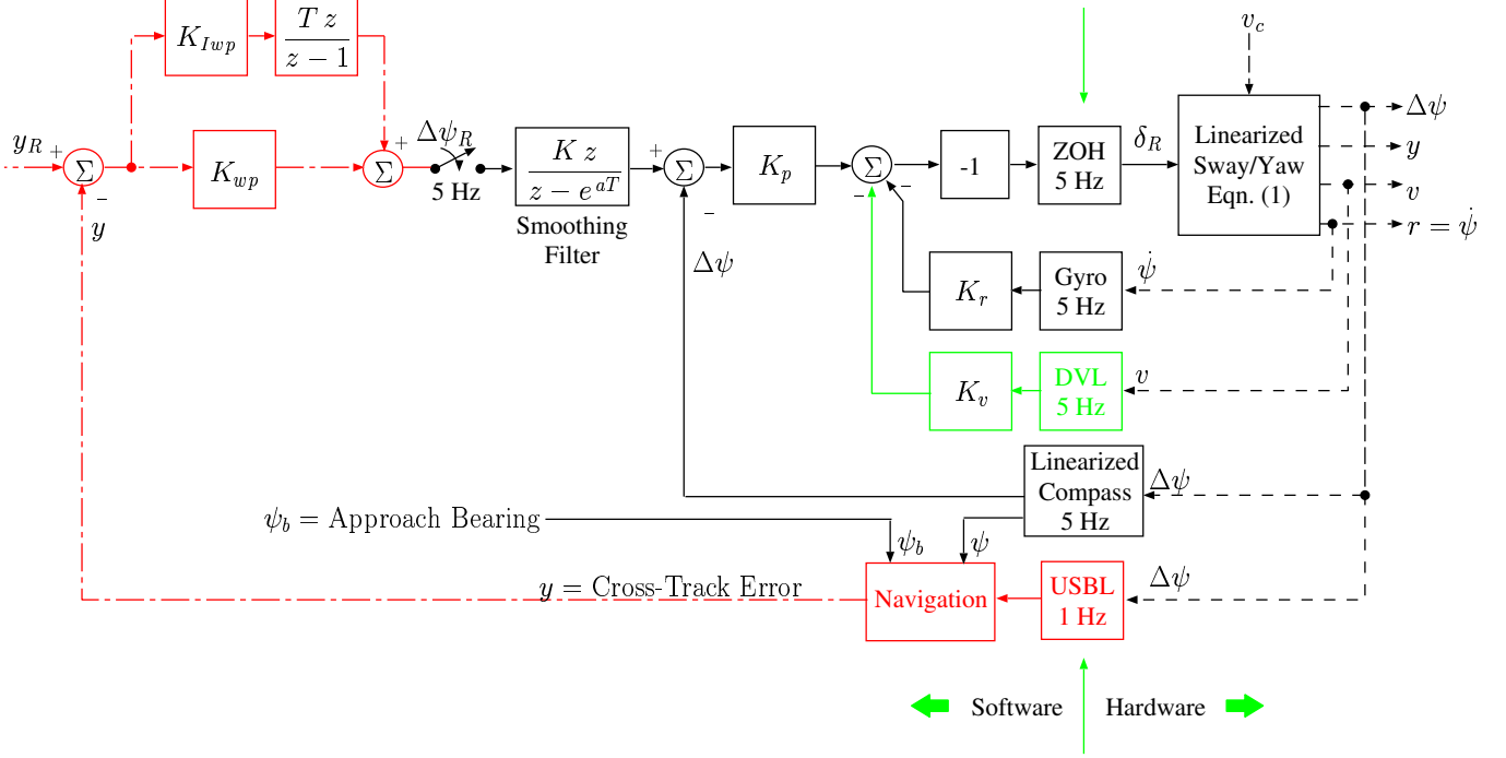
Fig. 8. Cross-track docking control loop. This system does not switch on until 200 m from the beacon. Consequently the outer USBL loop, shown with long and short dashes, runs at about 1 Hz, as opposed to the pure pursuit system in Fig. 6, where the vehicle may be as far as 2 km away when it acquires the beacon.
