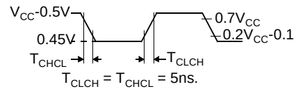
Figure 63. Clock Signal Waveform for I_{CC} Tests in Active and Idle Modes
