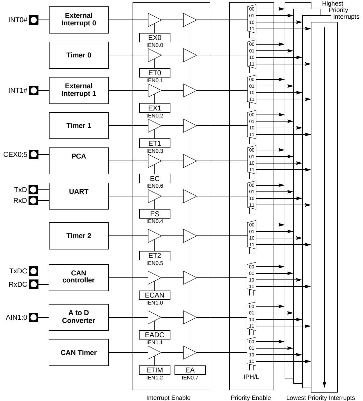
Figure 59. Interrupt Control System
