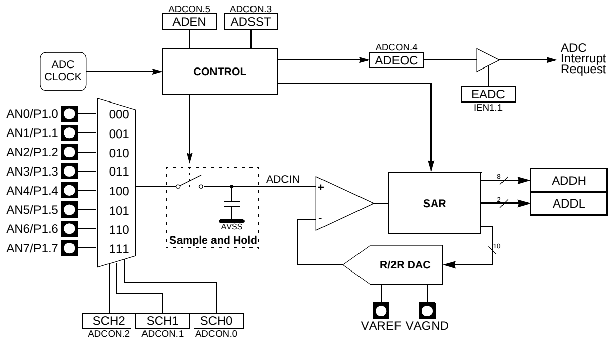
Figure 55. ADC Description
