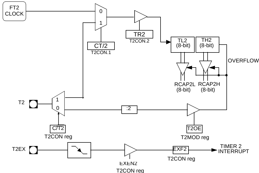
Figure 37. Clock-Out Mode
