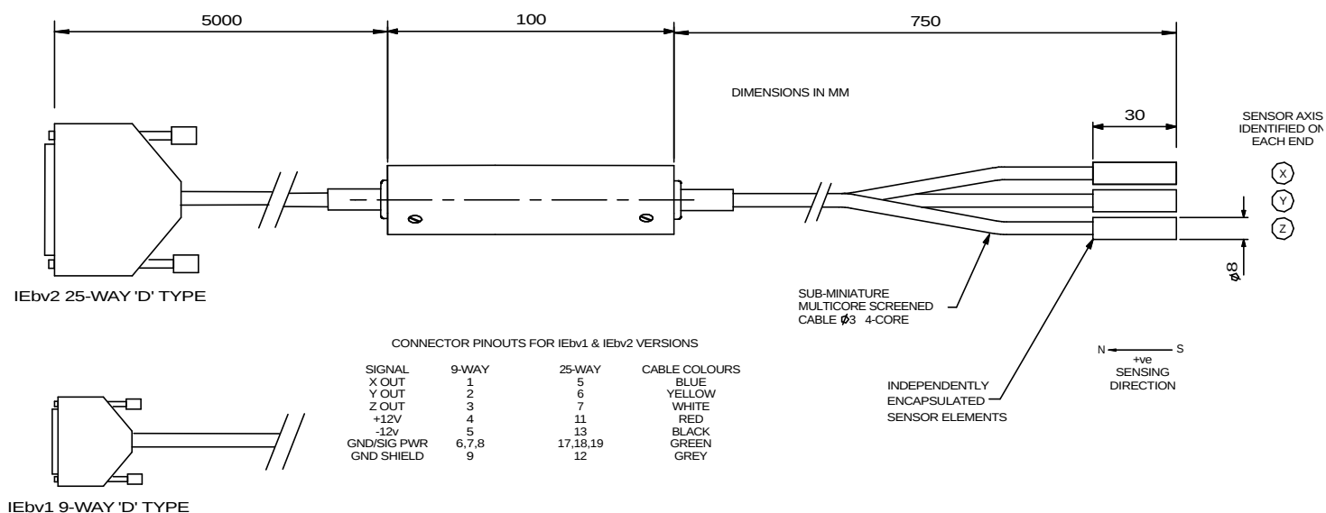
Figure 8 Mag-03IE ('D' TYPE CONNECTOR) V1, 9-WAY & V2, 25-WAY SENSOR OUTLINE DR1481(3)
