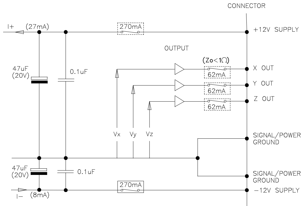
Figure 17 Mag-03 INTERFACE SCHEMATIC DR1006(2)
