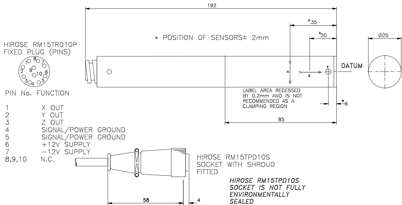
Figure 1 Mag-03MC SENSOR OUTLINE WITH MATING CONNECTOR DR0657(2)
