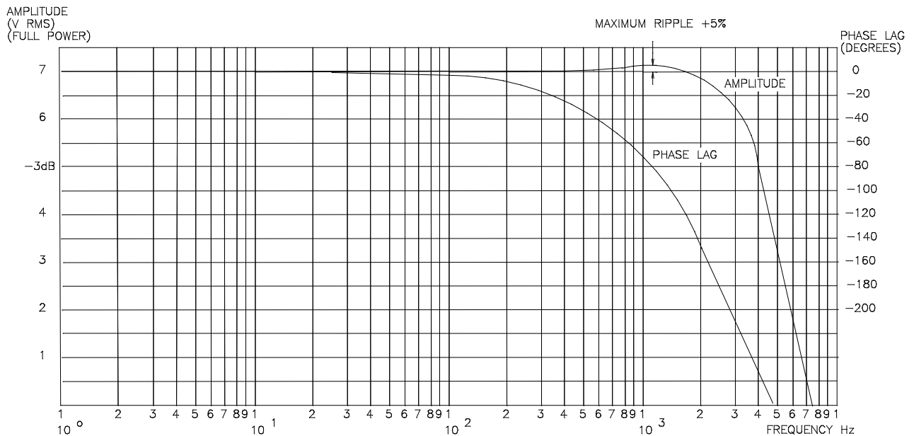
Figure 18 Mag-03 TYPICAL FREQUENCY DEPENDENT AMPLITUDE & PHASE RESPONSE DR1007(2)
