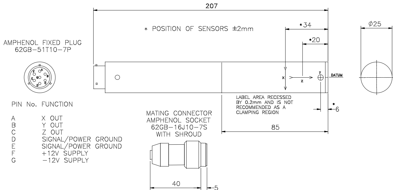
Figure 2 Mag-03MCES SENSOR OUTLINE WITH MATING CONNECTOR DR0656(2)
