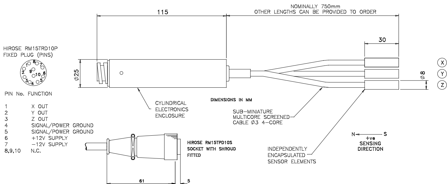
Figure 7 Mag-03IE ('HIROSE' CIRCULAR PLUG) SENSOR OUTLINE WITH MATING CONNECTOR DR0747(3)
