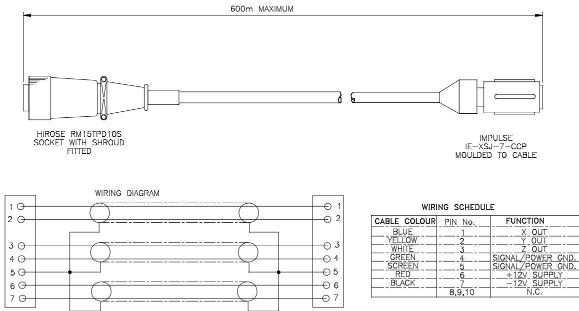
Figure 15 Mag-03MSS CABLE DR1017(2)
