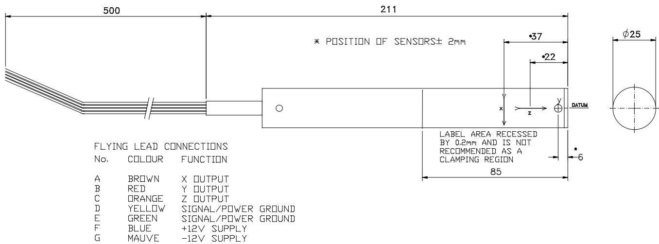
Figure 3 Mag-03MCFL SENSOR OUTLINE DR0745(2)
