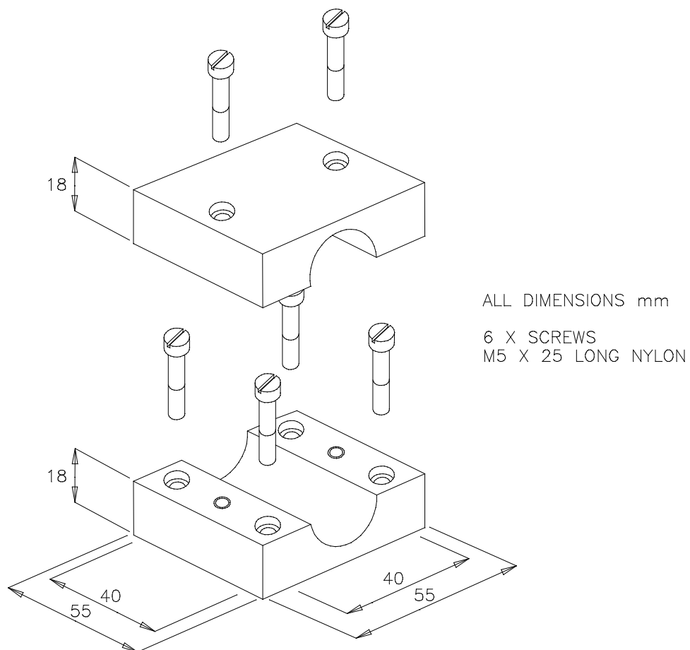
Figure 16 Mag-03MC-BR MOUNTING BRACKET DR0746(2)
