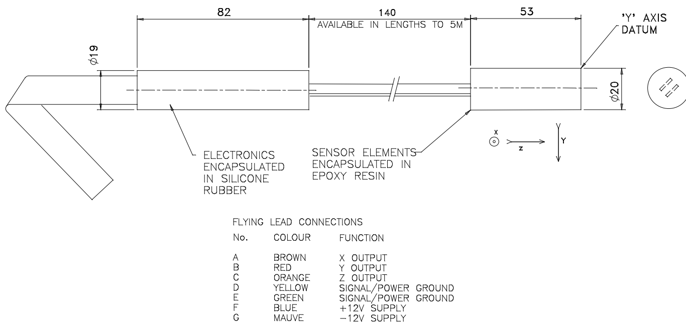
Figure 10 Mag-03MCUP VERSION SENSOR OUTLINE DR0758(2)
