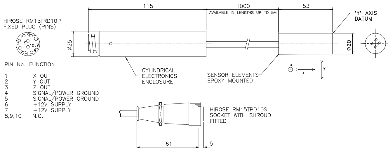
Figure 9 Mag-03MCTP VERSION SENSOR OUTLINE WITH MATING CONNECTOR DR0757(3)
