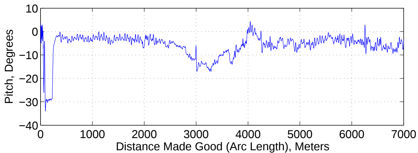
Vehicle Pitch
