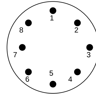
ODI Pin Numbering (looking in at pins)
