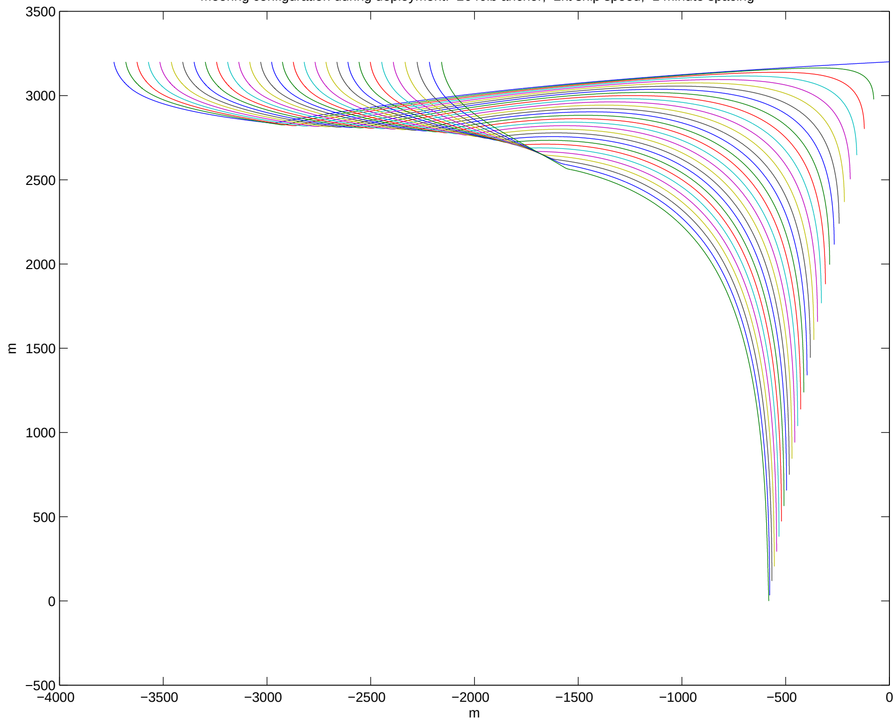
Mooring configuration during deployment. 2640lb anchor, 2kt ship speed, 1 minute spacing
