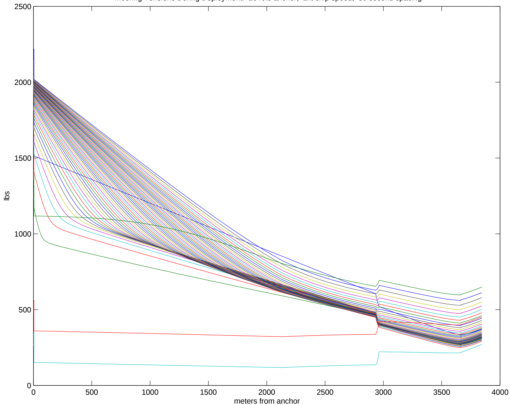
Mooring Tensions During Deployment. 2640lb anchor, 2kt ship speed, 30 second spacing
