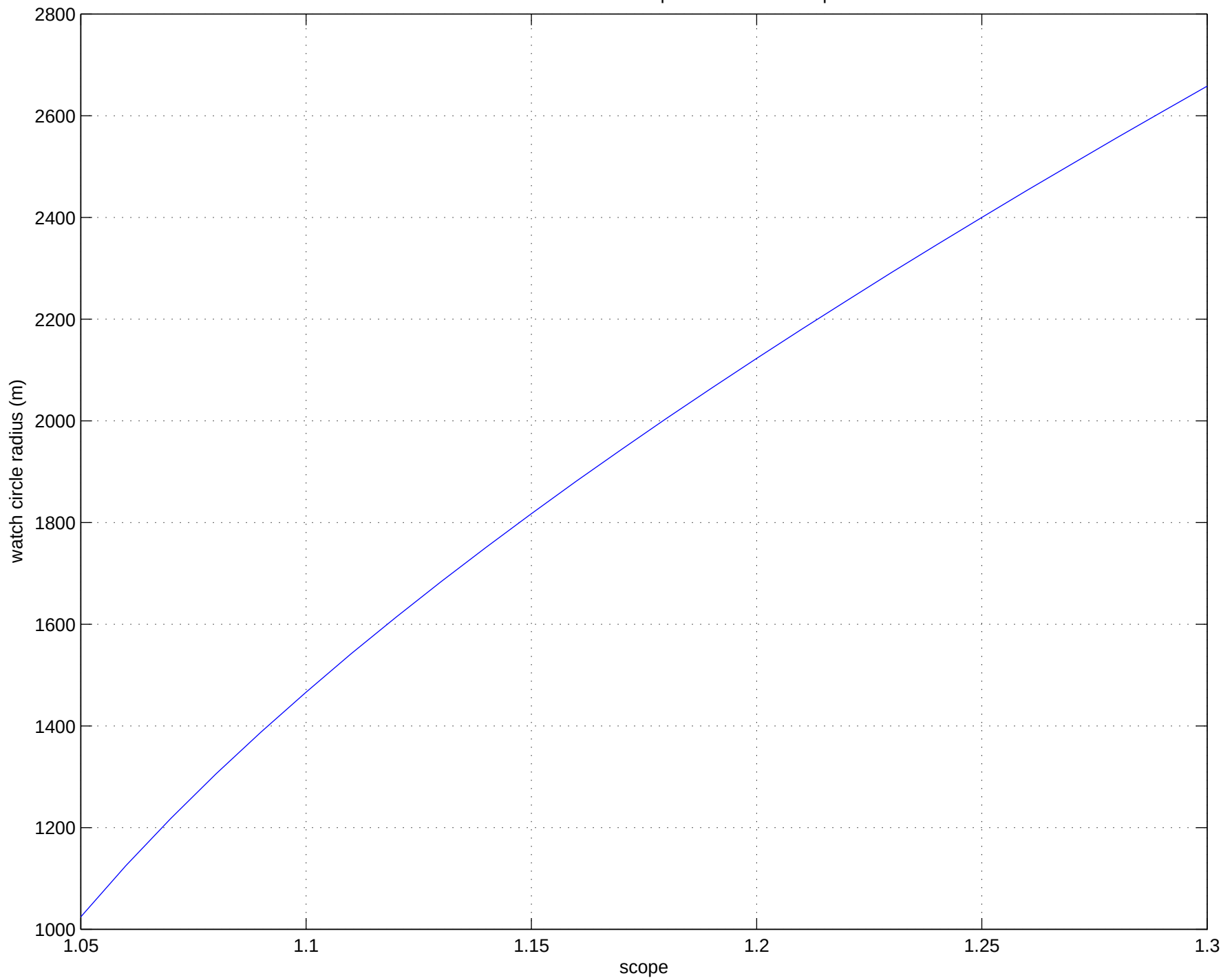
Watch circle radius vs. scope: 3200m water depth
