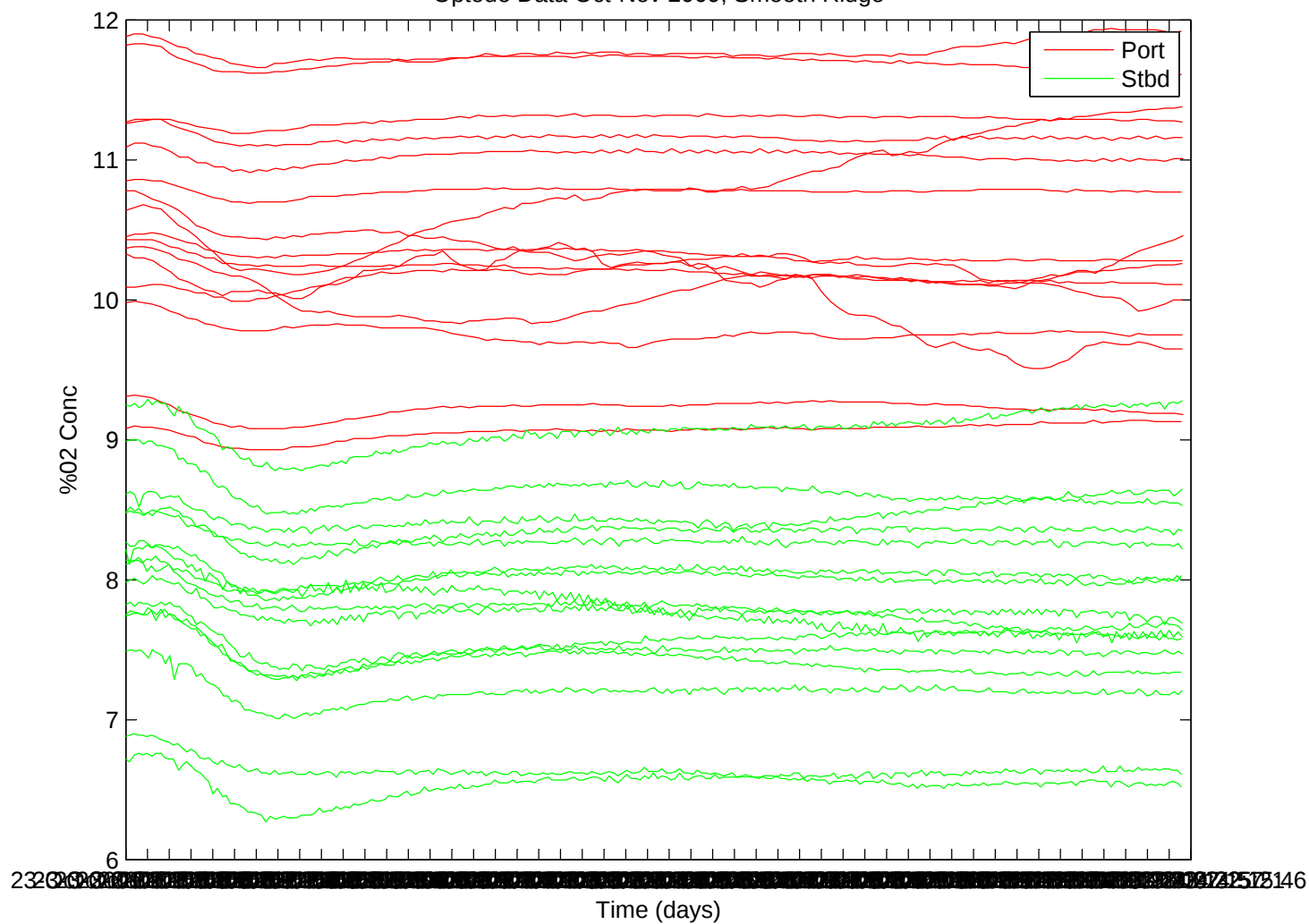
Optode Data Oct-Nov 2009, Smooth Ridge
