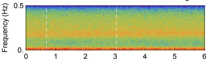
MOBB Seismometer Differential Pressure Gauge
