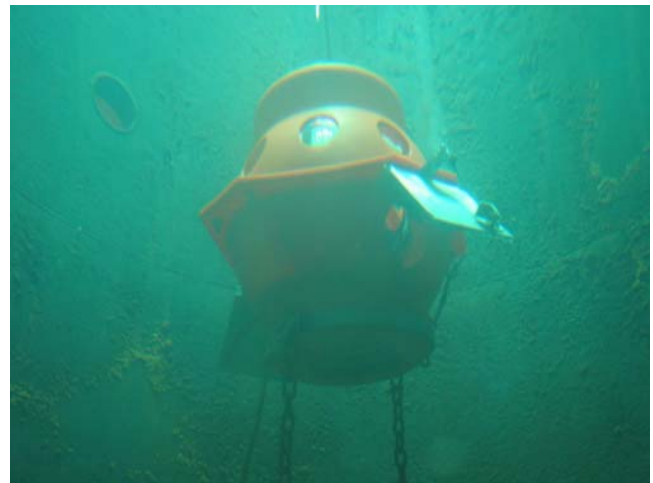
Fig. 3. DOVE full-up test in Scripps Institution's 10m Deep Tank. Fins are the flash reflectors. Chains connect to the release collar at the base. Upper holes allow more light from the recovery strobe to get through. A trail of bubbles to the right is coming from the active burnwire release system.
