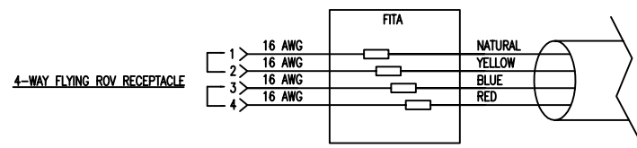
WIRING DIAGRAM
