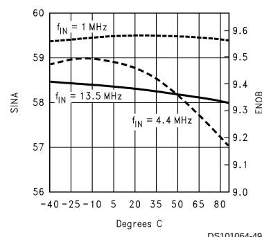
SINAD & ENOB vs Temperature and f_{IN}
