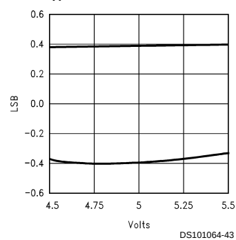
INL vs V_A
