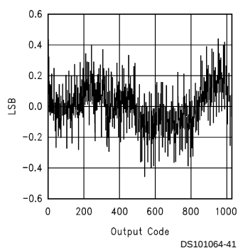
Typical INL
