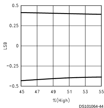
INL vs Clock Duty Cycle
