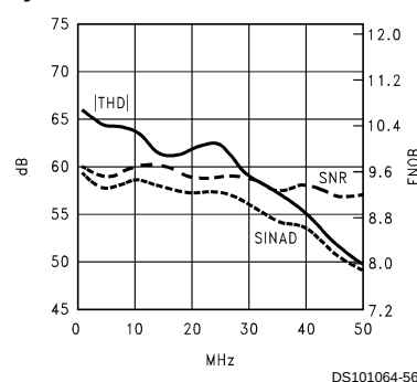
Dynamics at 30 MSPS
