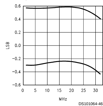
DNL vs f_{CLK}
