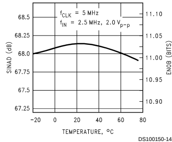
SINAD vs Temperature
