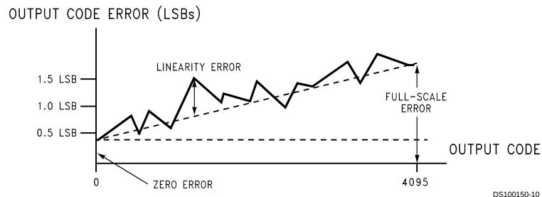
FIGURE 2. Errors Minimized by the Auto-Cal Cycle
