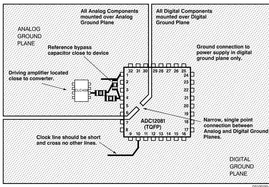
FIGURE 6. Layout example
