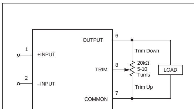
Figure 2a. Trim Connections Using a Trimpot
