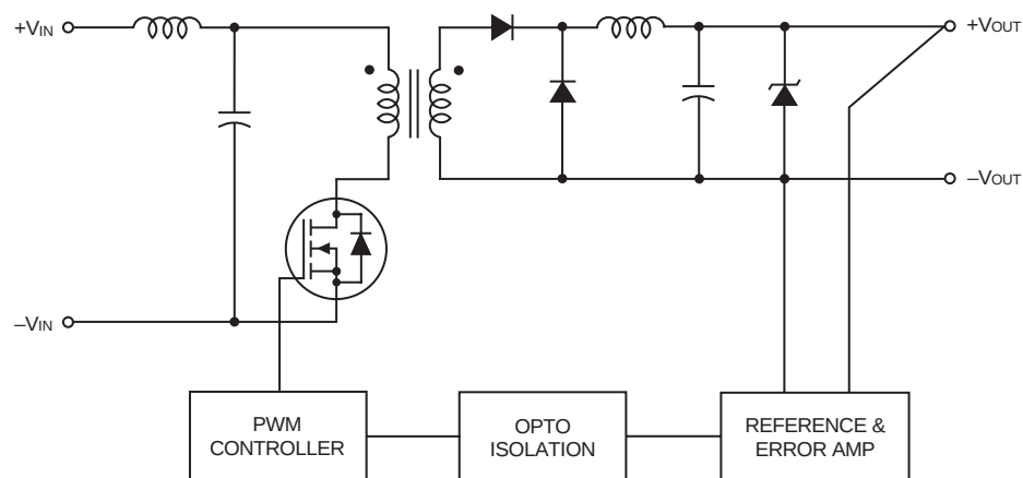
Figure 1. Simplified Schematic
