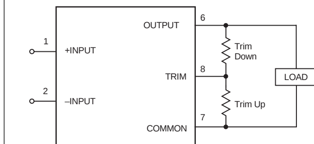
Figure 2b. Trim Connections Using Fixed Resistors
