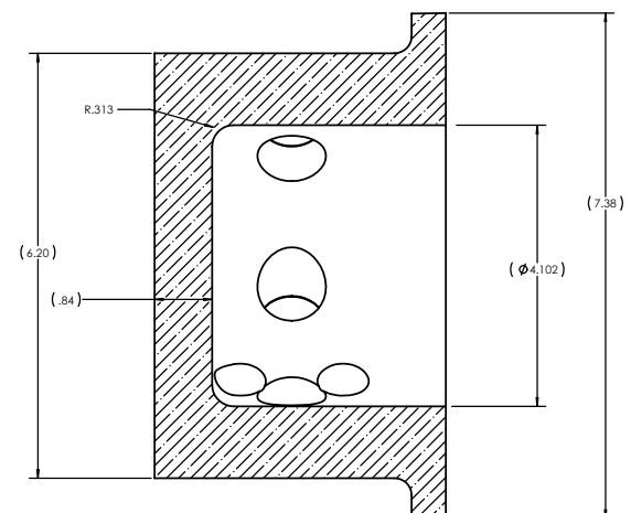
SECTION K-K
