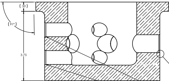
SECTION L-L
