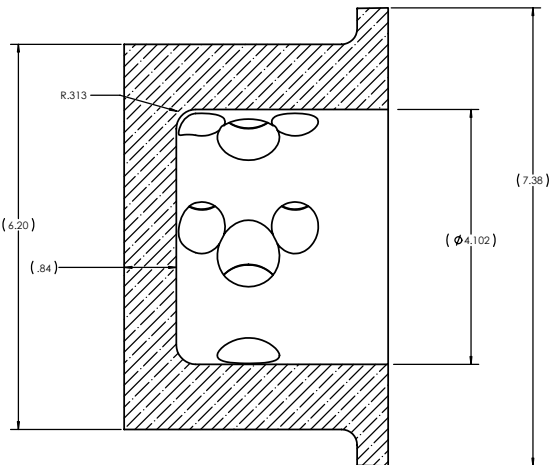
SECTION K-K
