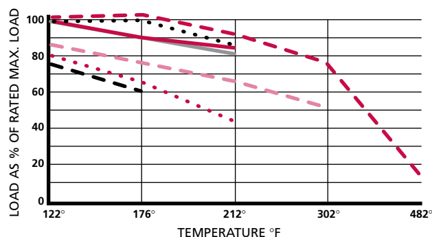
Fig 2: Capacity vs temperature
