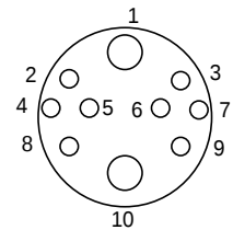
Seacon MINK 10 CCPL TI FEMALE FACE
