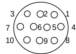
MINM 10 CCPL Face view of male connector
