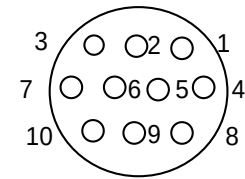
MINM 10 CCPL Face view of female connector
