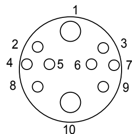
Seacon MINK 10 CCPL TI FEMALE FACE
