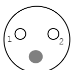
Subconn MCBH2M Face View
