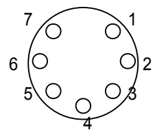
Impulse MIL-7-MP MALE FACE VIEW
