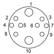
Seacon MINK 10 CCPL TI FEMALE FACE
