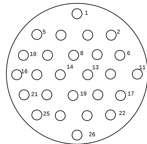
Face View Of Seacon MINM26 CCP
