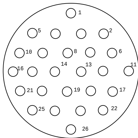
Face View Of Seacon MINM26 CCP
