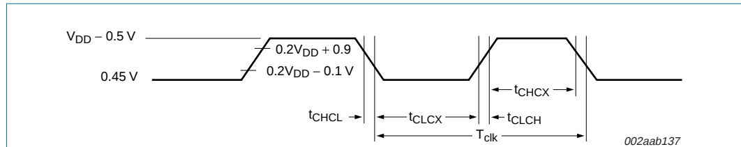
Fig 7. External clock timing.
