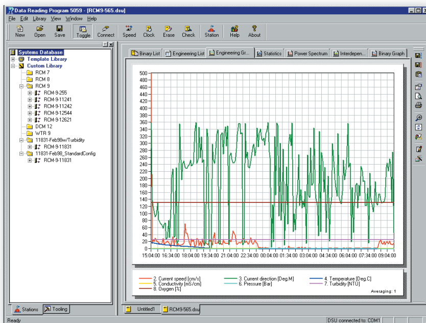
Engineering Data graph from RCM 9 serial. no. 565
