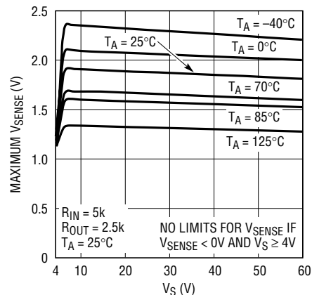
Input Sense Range vs Supply Voltage
