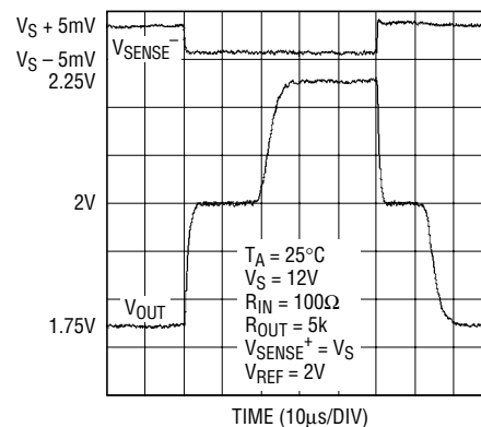
Step Response -5mV to 5mV
