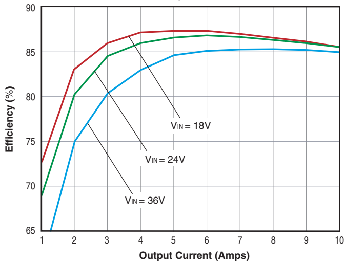
UHE-1.5/10000-D24 Efficiency vs. Load @ +25°C Ambient
