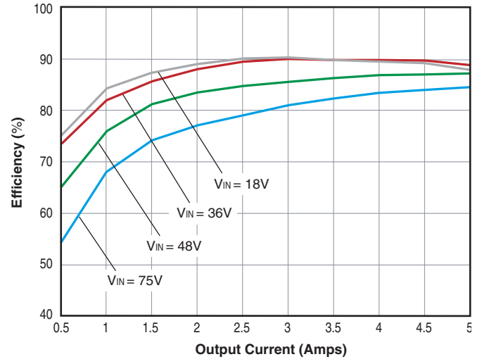
UHE-5/5000-Q48 Efficiency vs. Load @ +25°C Ambient
