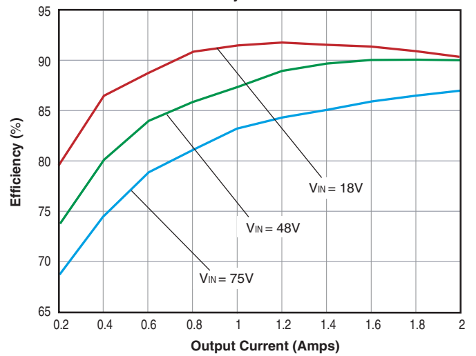
UHE-15-2000-Q48 Efficiency vs. Load @ +25°C Ambient
