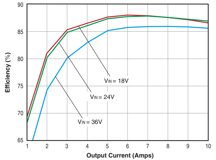
UHE-1.8/10000-D24 Efficiency vs. Load @ +25°C Ambient
