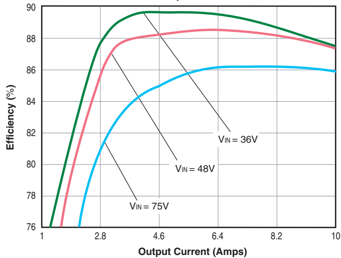
UHE-2.5/10000-D48 Efficiency vs. Load @ +25°C Ambient
