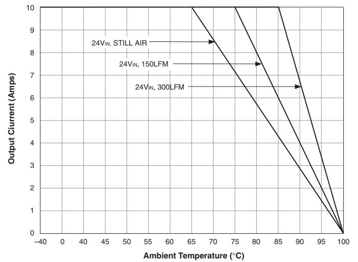
UHE-1.8/10000-D24 Temperature Derating
