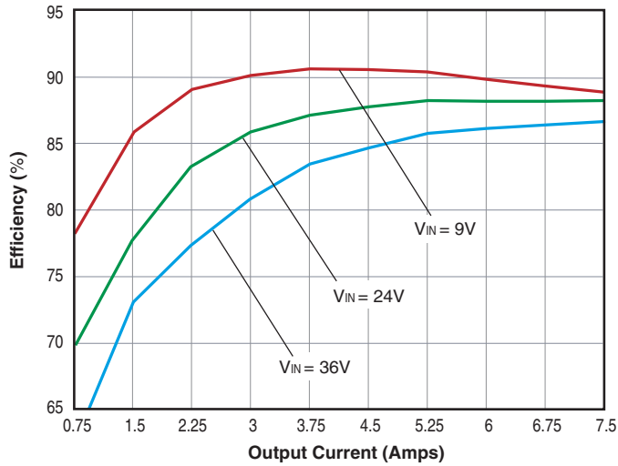
UHE-3.3/7500-Q12 Efficiency vs. Load @ +25°C Ambient
