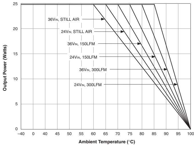
UHE-3.3/7500-Q12 Temperature Derating
