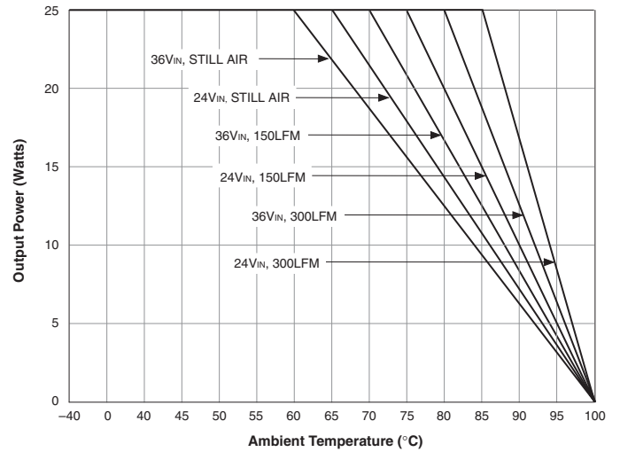
UHE-5/5000-Q12 Temperature Derating
