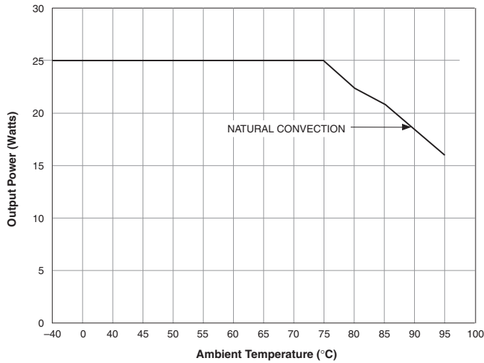
UHE-2.5/10000-D48 Temperature Derating
