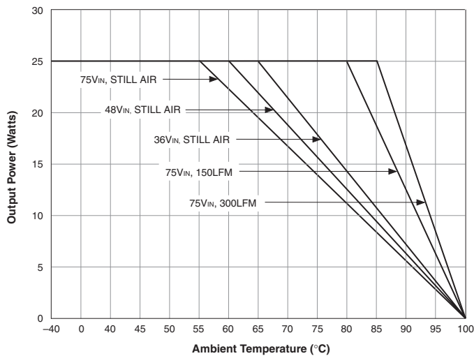
UHE-3.3/7500-D48 Temperature Derating
