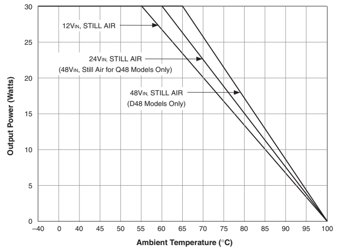
UHE-12/2500 and UHE-15/2000 (All Models) Temperature Derating
