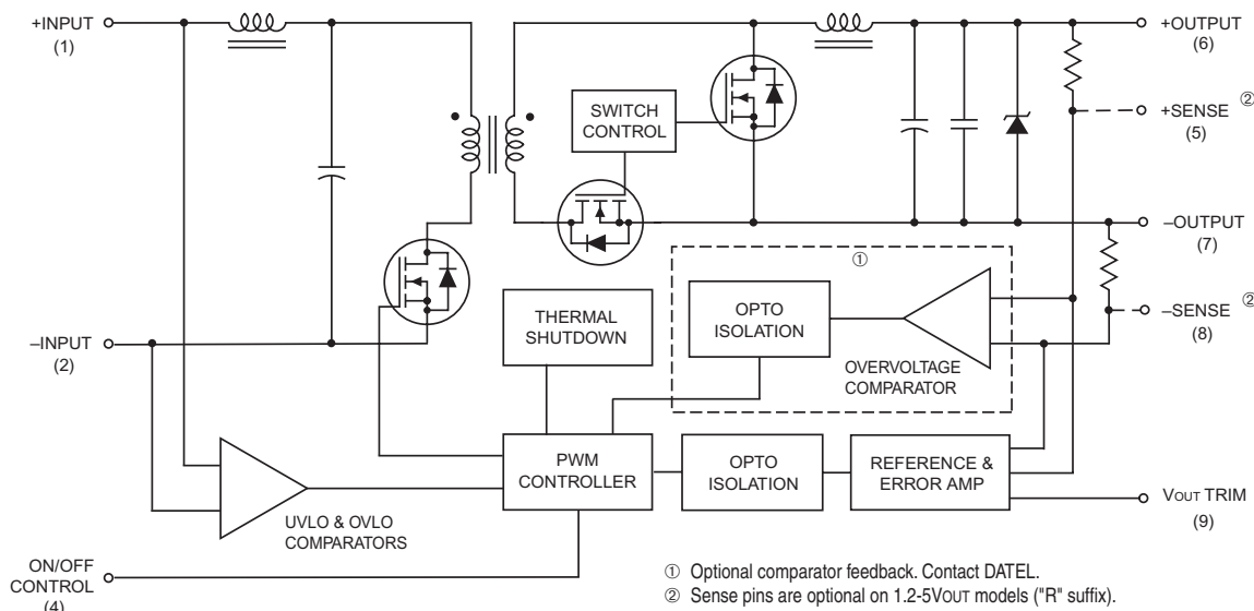
Figure 1. Simplified Schematic
