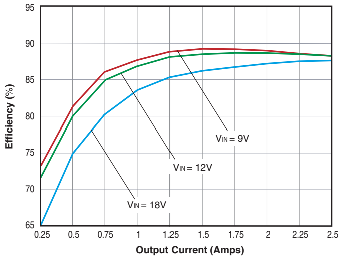
UHE-12/2500-D12 Efficiency vs. Load @ +25°C Ambient
