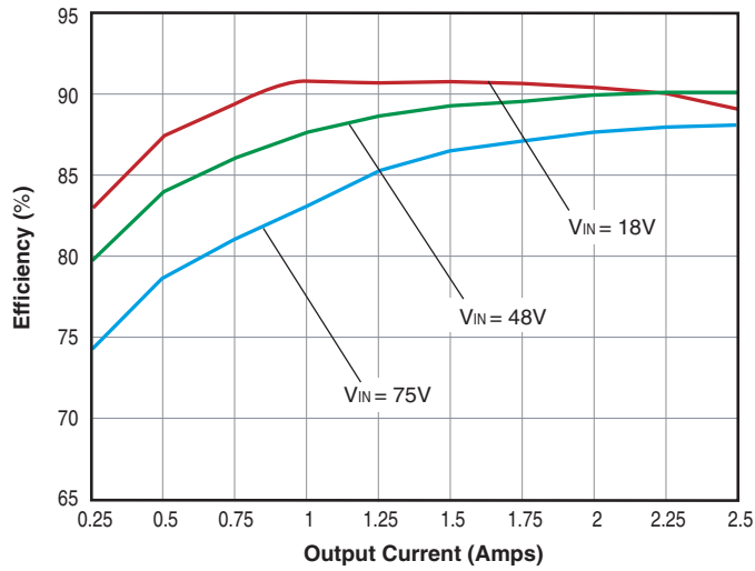
UHE-12-2500-Q48 Efficiency vs. Load @ +25°C Ambient
