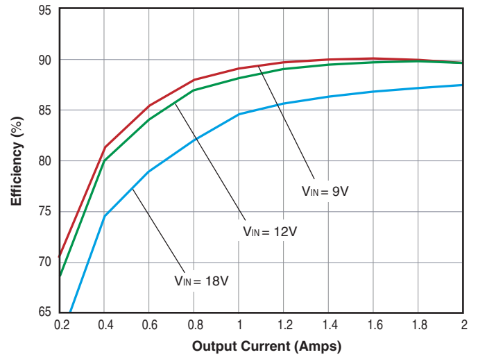
UHE-15/2000-D12 Efficiency vs. Load @ +25°C Ambient
