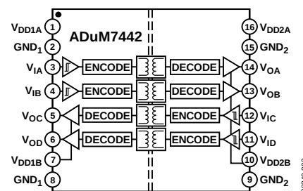
Figure 3. ADuM7442
