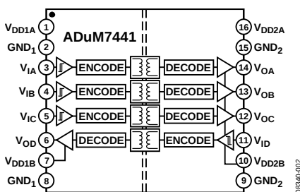
Figure 2. ADuM7441
