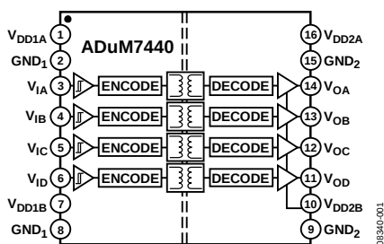
Figure 1. ADuM7440
