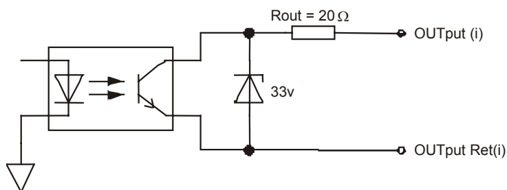
Figure 3: Digital Output Schematic
