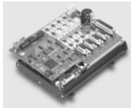
SDM-20640 Interconnect with 4-axis microstep drives
