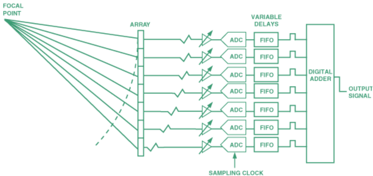
Figure 5. Simplified block diagram of DBF system.
