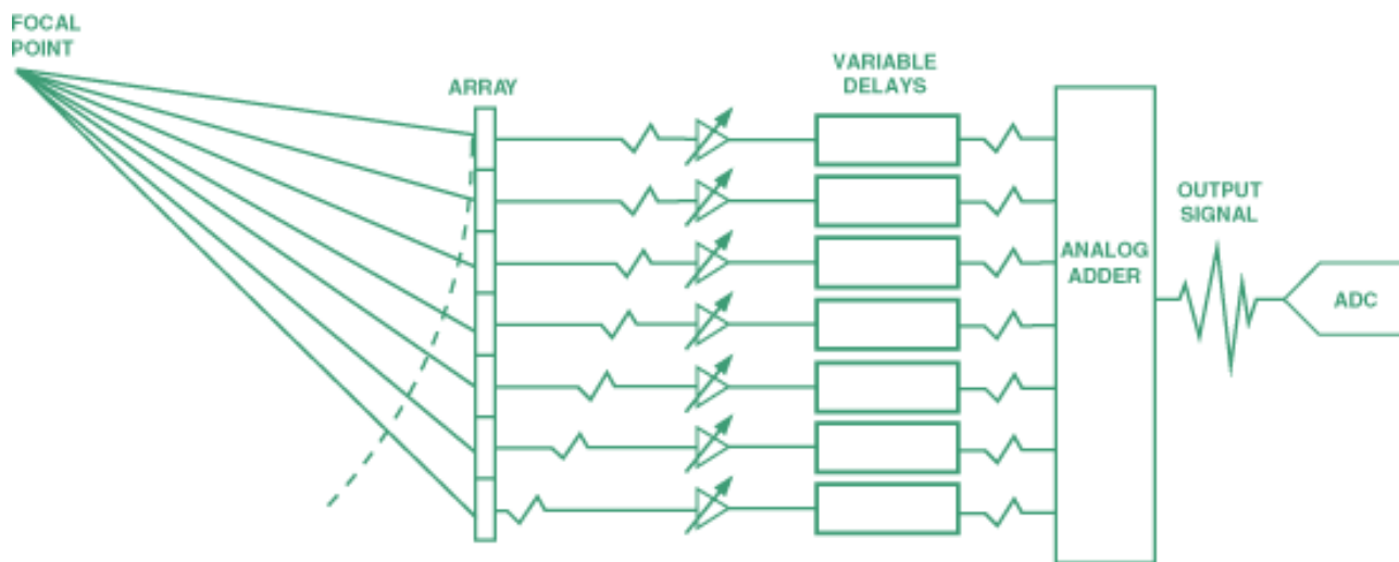
Figure 4. Simplified block diagram of ABF system.
