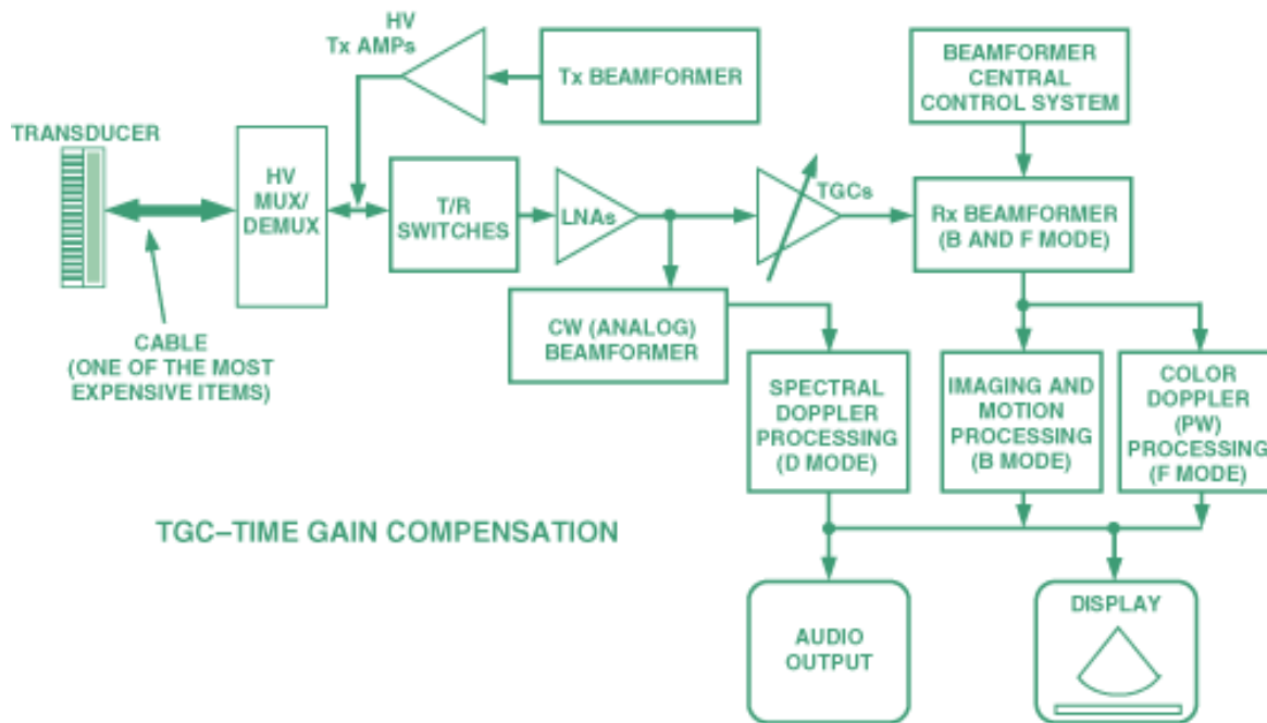
Figure 1. Ultrasound system block diagram.
