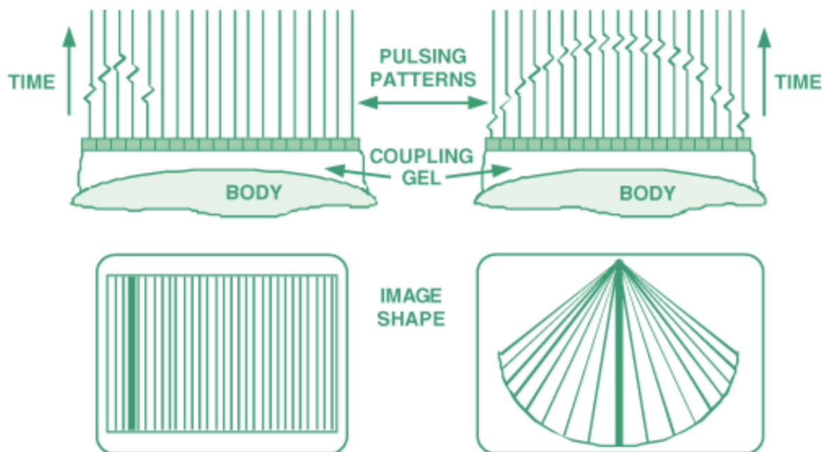
Figure 3. Linear vs. phased-array imaging.
