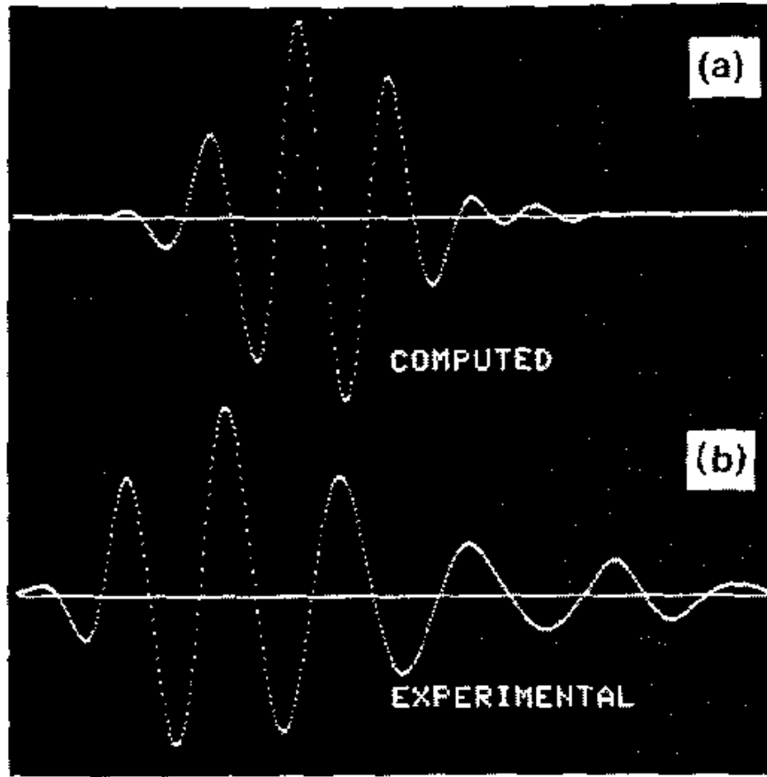
Figure 3: Pulses for medical ultrasound. (a) Model pulse used in computer generation of beam response. The pulse represents the voltage echo response from a very short pulse electrical input. As far as can be ascertained, the pulse represents the true point echo response. (b) Actual experimental voltage echo off a nylon line in water. The ringing is due to the line's not being a point. Figure reproduced from Robinson and Wing [1984].
