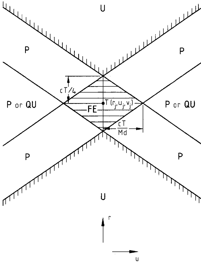
Figure 24: Showing regions in the image of a point target located at T . Image points have coordinates (r, u, v) ; the 'plane' v = \text{constant} is shown. FE=fully-enisonified region, U=umbra or full-shadow region, P=penumbra, QU=quasi-umbra.
