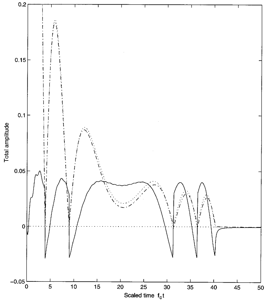
Figure 29: Total amplitude Y_t of the autocorrelation function, for \beta = 1/3.5 , f_c T = 40.25 (dash-dot). Also shown are the program's approximation (dotted) and 10 times the program's error (continuous). m = 32\,768 , \theta = 1/14 .
