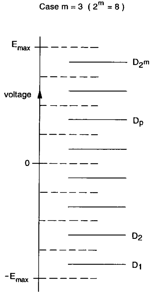
Figure 15: Quantisation. The uniformly quantised region (-E_{\max}, E_{\max}) is subdivided into 2^m equal intervals. The allowed output values D_p are the midpoints of these intervals.
