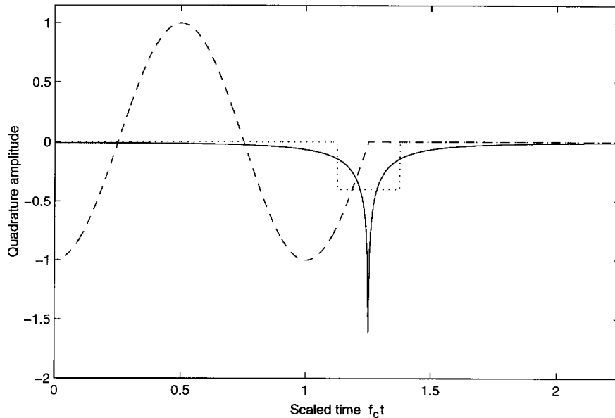
Figure 28: Error in the quadrature amplitude, due to the program, from the step-function-end data shown in Figure 27. Shown are the program's approximation (dashed), the error (continuous) and a rough approximation to the error (dotted). The latter approximation consists of a single rectangle function of height 0.40 and width 0.25.
