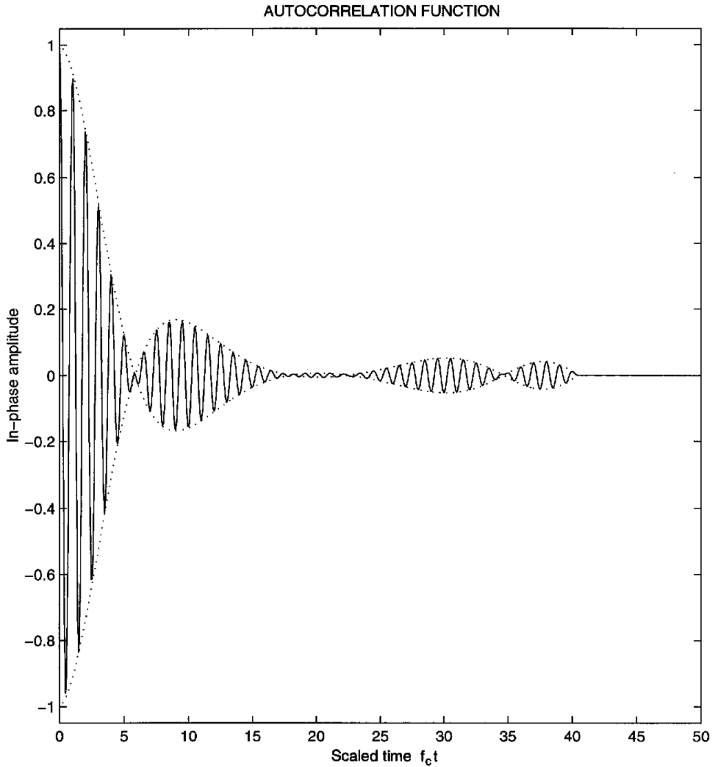
Figure 11: In-phase autocorrelation function Y(t) (continuous) for \beta = 1/5 , f_c T = 40.5 . The envelope of the program's approximation is also shown (dotted). Processing parameters: m = 4096 , \theta = 1/8 .
