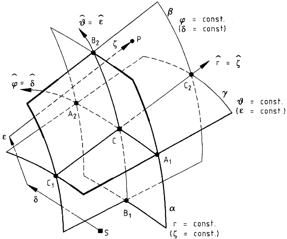
Figure 10: The viewwindows for the unrotated radially-curved case. For linear plots the viewwindows are A_1CA_2 , B_1CB_2 and C_1CC_2 . For planar plots the viewwindows are the three intersecting curved ‘rectangles’. The path from S to P is the same as in Figure 2. The significance of the secondary origin S is that, on the graphs, the coordinate labels are proportional, not to \phi , \theta and r , but to \phi - \phi_s , \theta - \theta_s and r - r_s , where the subscript s refers to the point S . Indeed the labels themselves are numerically equal to \delta , \epsilon and \zeta .
