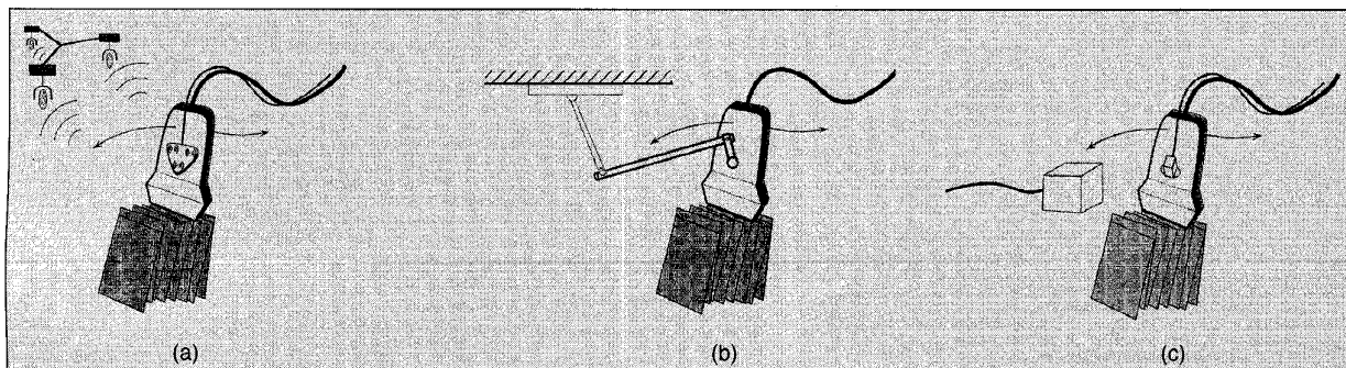
2. Schematic diagram showing three basic methods for obtaining the position and orientation of the ultrasound transducer for the free-hand acquisition technique: a) acoustic, b) articulated arm, and c) electromagnetic positioners.
