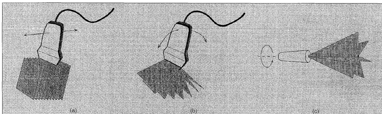
3. Schematic diagram showing the three basic types of motion used in 3-D ultrasound systems making use of mechanical scanning: a) linear, b) fan, and c) rotational.
