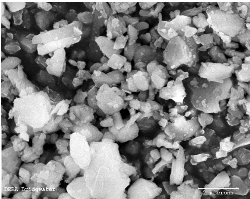
Figure 5. SEM image of Polcarb (calcium carbonate) particles using an original instrument magnification of \times 10\,000 .
