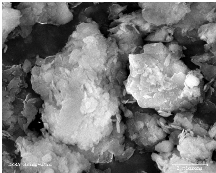
Figure 8. SEM image of marine sediment particles using an original instrument magnification of \times 10\,000 .
