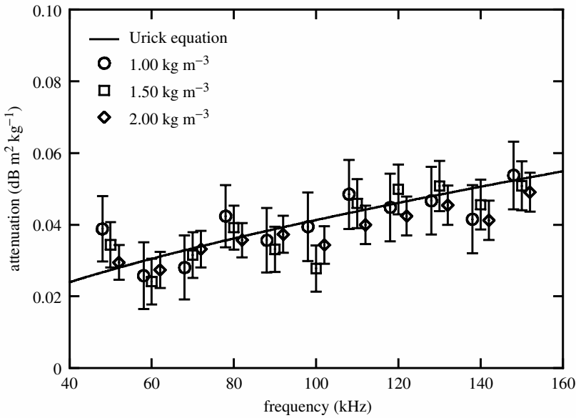
Figure 3. The normalized attenuation coefficient for spherical particles: experimental data and theoretical predictions using Urlick's equation. The data points have offsets in frequency as described in the text.
