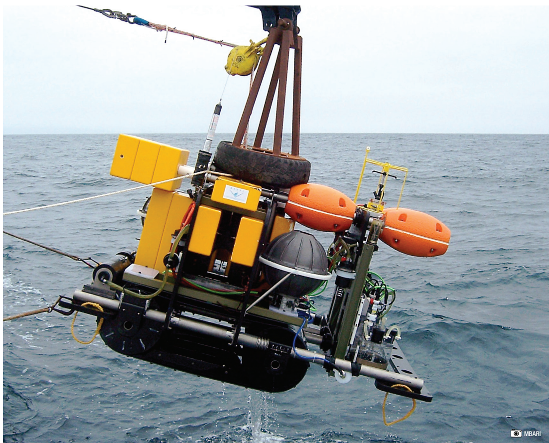
Figure 1: The Rover during recovery operations after a deployment in Monterey Bay.
