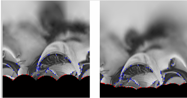
Fig. 3. Extracted features are shown. The red features, which are the border features, are removed automatically before applying RANSAC.
