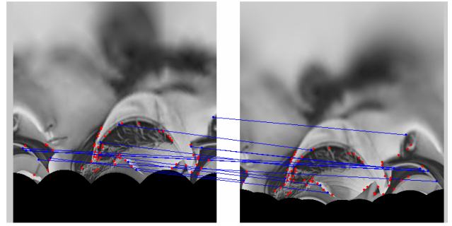
Fig. 4. Features are matched. The inliers are shown in blue. The red features are the outliers.
