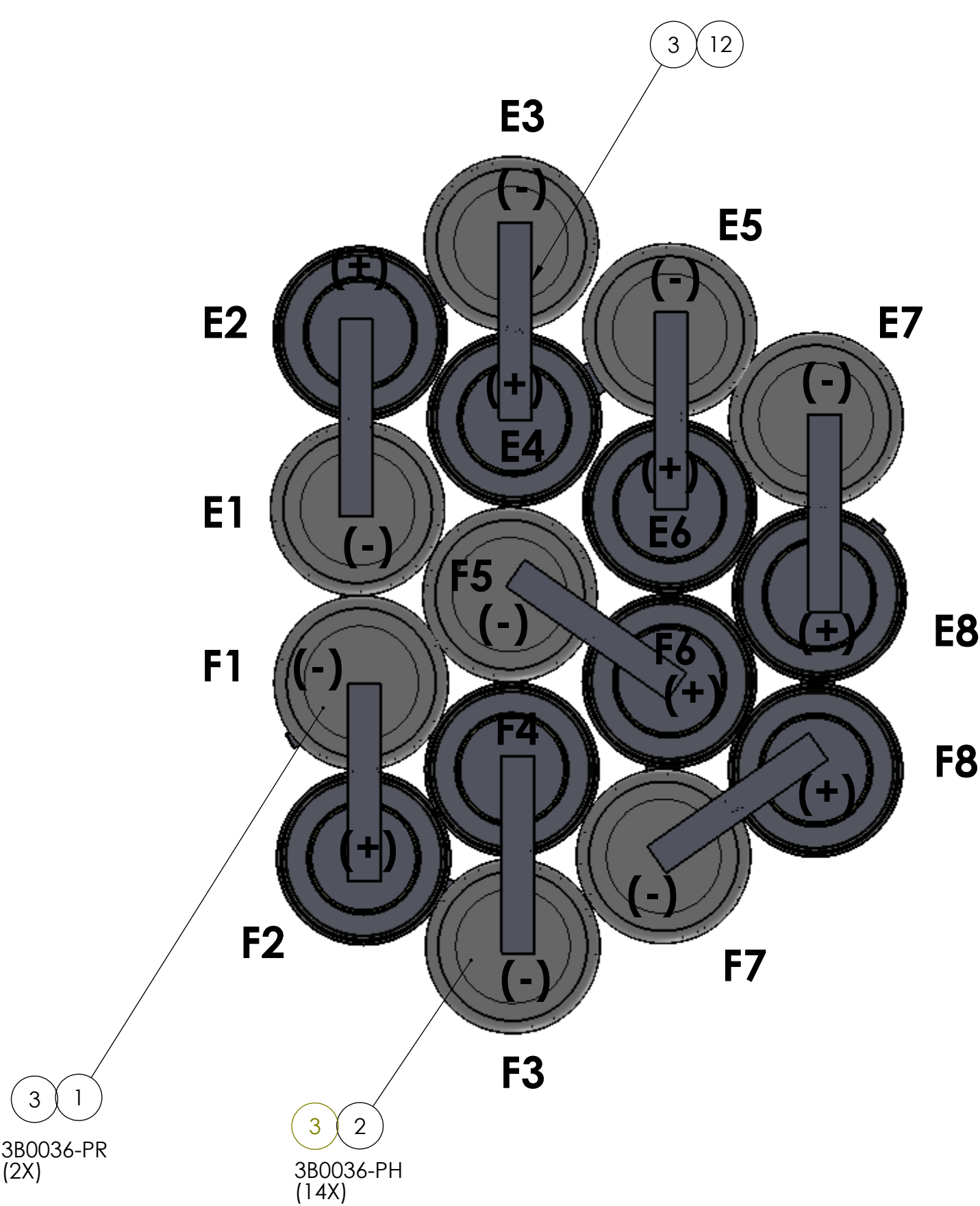
BOTTOM VIEW SHOWN WITHOUT INSULATOR, HEATSHRINK, TAPE
