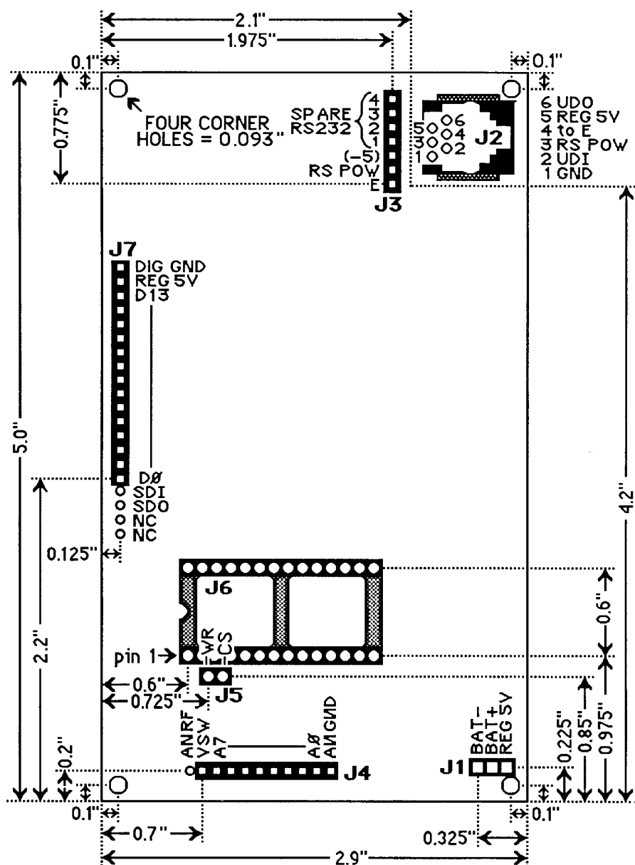
Tattletale Model II Dimensions
