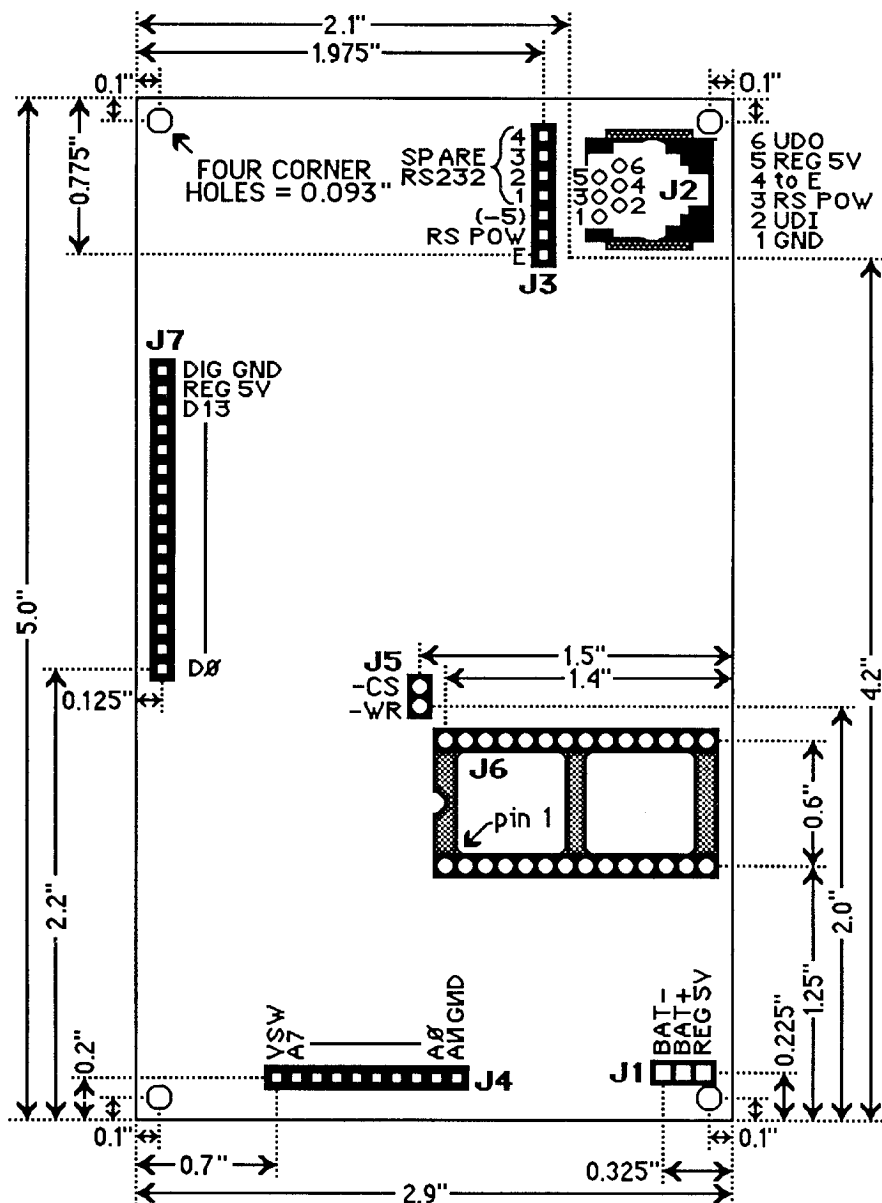
Tattletale Model III Dimensions
