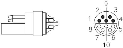
10 PINS INSERT, EXTERIOR VIEW
