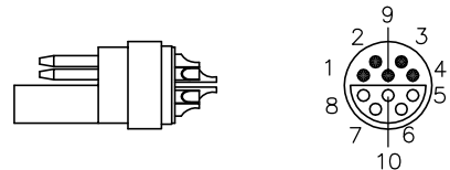
10 PINS INSERT, EXTERIOR VIEW
